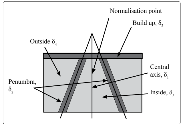
Fig. 1. Definition of different regions in a radiation beam, based on the magnitude of the dose and dose gradient (Adapted, from ESTRO report [6] ).
