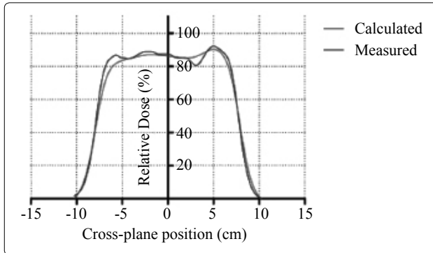
Fig. 3. Comparison between measured and calculated dose profiles for 16 MeV electron beam (CT based Inhomogeneity corrections tests With Gafchromic EBT2 film).
