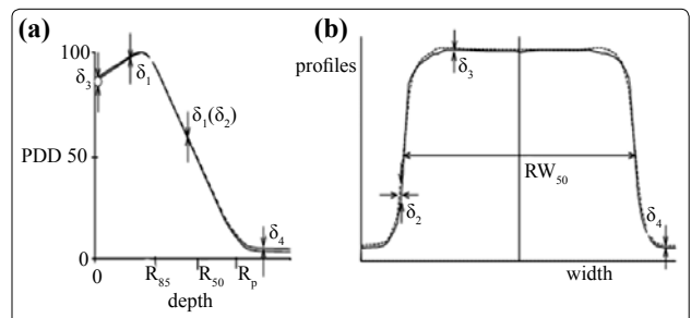
Fig. 2. Different tolerances are proposed for the various regions in a electron beam; (a) depth-dose curve; (b) beam profile (Adapted, from ESTRO report [6] and NCS report [7] ).
